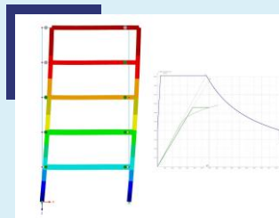
Pushover-Analysis
