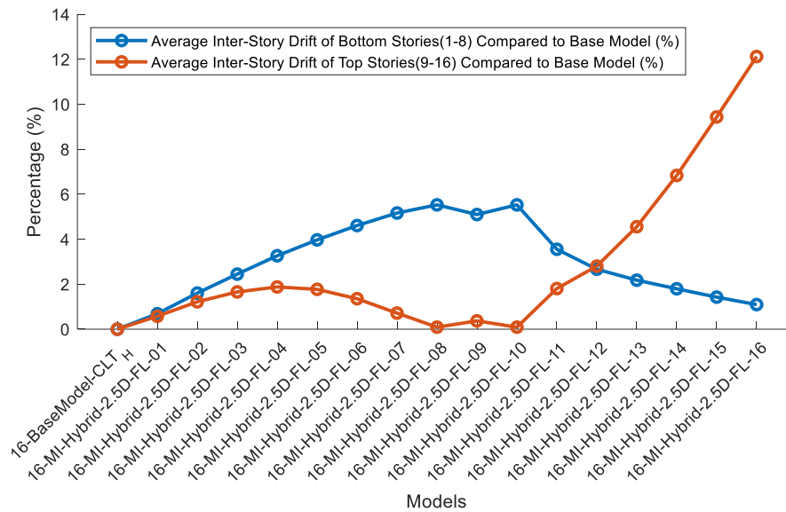
Fig. 6-2 Averaged Inter-Story Drift Variation (Top Stories vs. Bottom Stories) with Increased Mass Distribution along the Hybrid Structures
