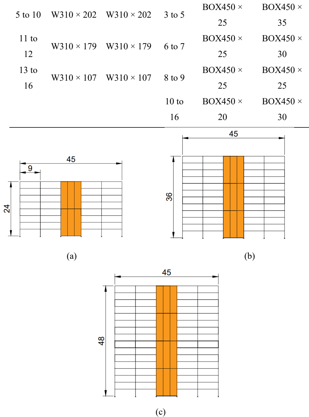
Fig. 3-4 Vertical Elevation: (a) 8-Story, (b) 12-Story, (c) 16-Story
