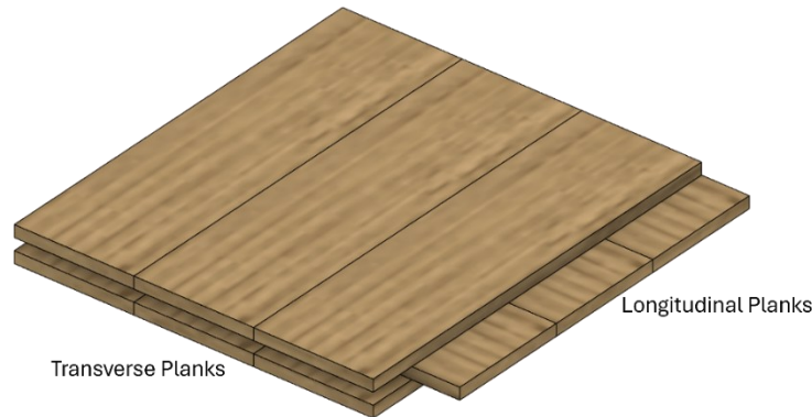
Fig. 1-1 CLT Panel Configuration
