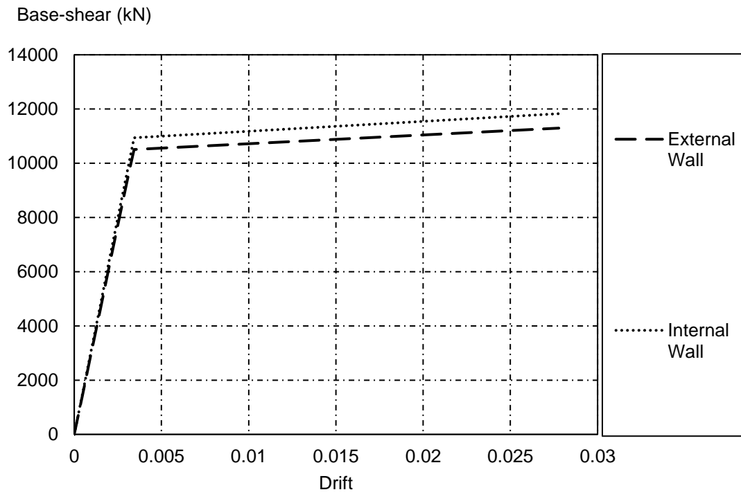
Figure 4-5: Results of pushover analysis: Base-shear vs Drift
