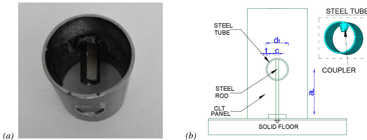
Figure 7-1: (a) Steel tube connector photo (Photo credit Mpidi Bita); and (b) Schematic representation of steel tube detailing
