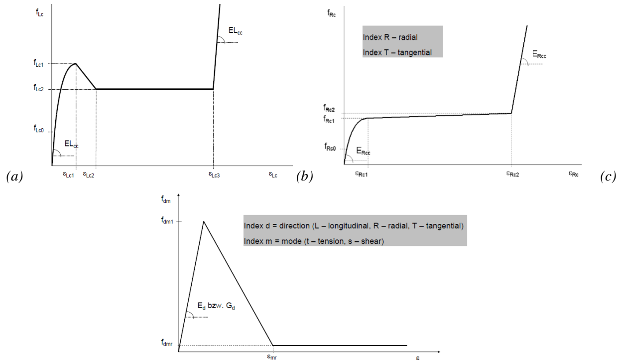
Figure A.3.1: (a) Uniaxial stress-strain curve of timber model in longitudinal compression; (b) Radial or tangential compression; and (c) Shear failure and tensile failure (Dynardo, 2016)
