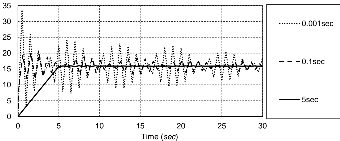
Figure 5-7: Effects of speed of element removal
