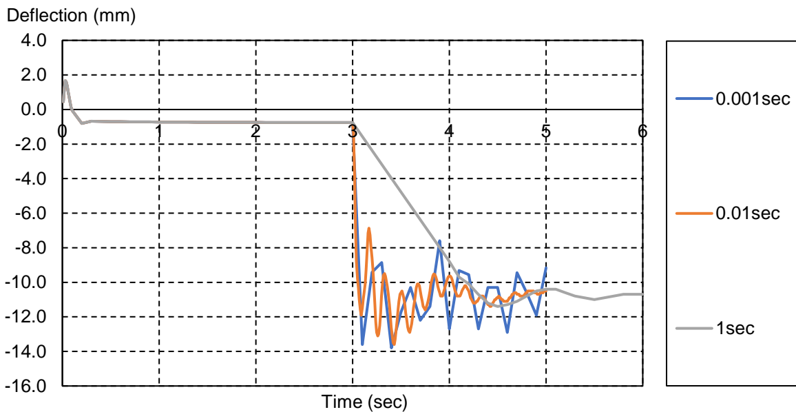
Figure 4-12: Effects of removal speed ( t_r )
