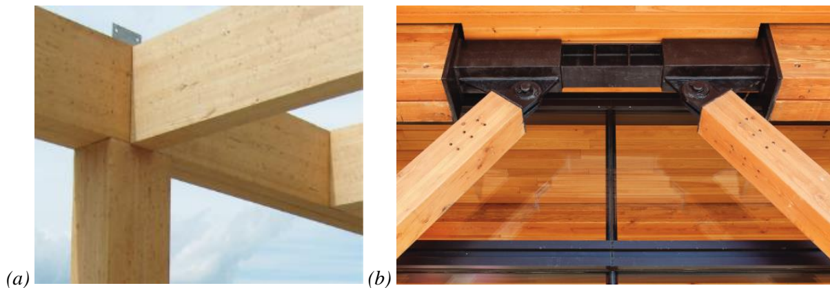
Figure 1-5: Post and beam mass-timber building: (a) Gravity load-resisting system; and (b) Lateral load-resisting system (Photo credit Matthew Millman)
