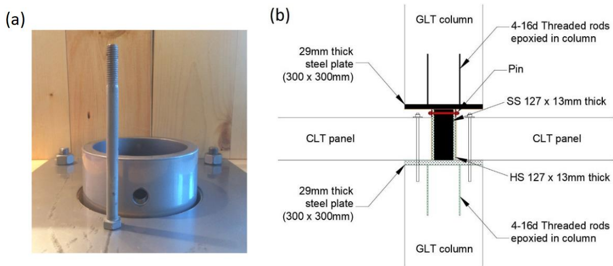
Figure 5-4: Column-to-column detailing: (a) Photo (Photo credit Mpidi Bita); (b) Schematic representation (Fast and Jackson, 2017)
