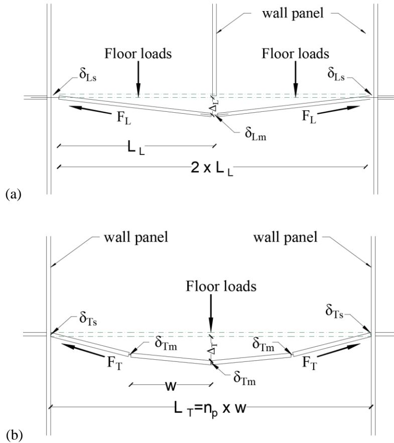
Figure 6-2: Floor system resistance mechanisms: (a) Catenary action after the loss of interior loadbearing walls; and (b) Catenary action after the loss of external loadbearing wall (as per Figure 2-5b)
