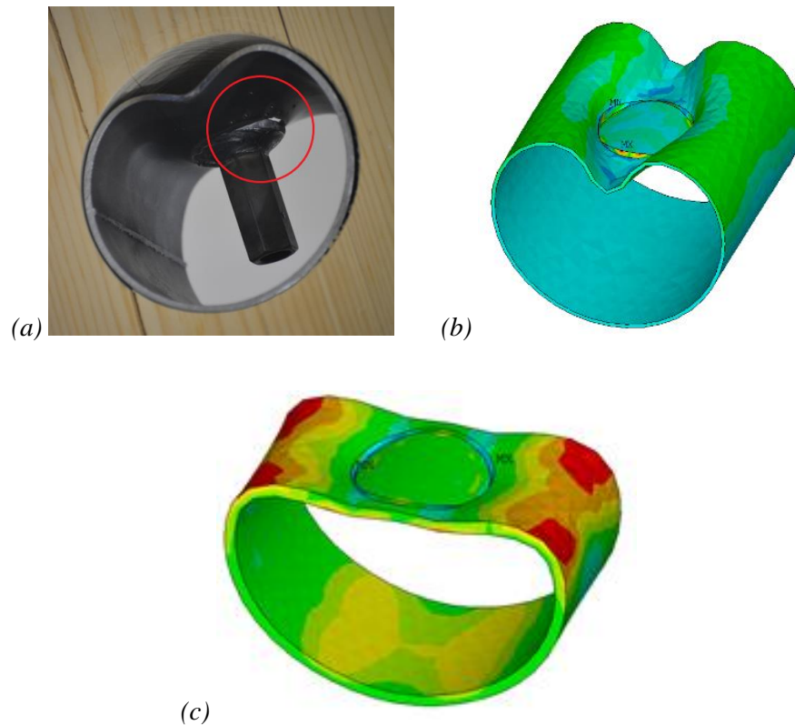
Figure 7-9: Failure modes: (a) Experiment; (b) Tube buckling; and (c) Tearing at weld-coupler
