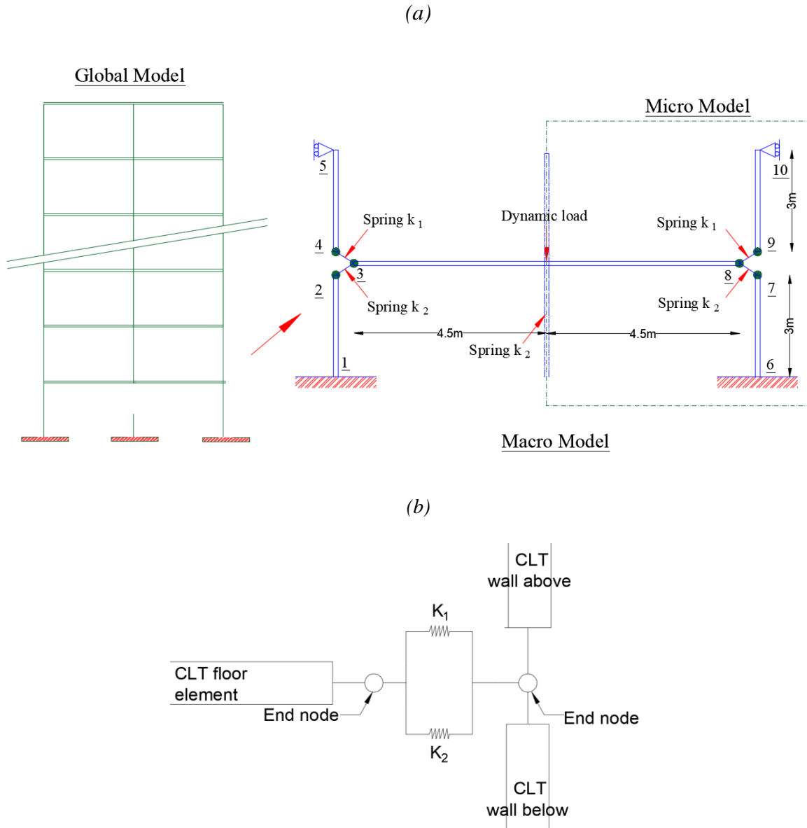
Figure 4-3: (a) Multi-level structural idealisation: Global model, Macro model, and Micro model (half of the Micro model); and (b) Micro model idealisation
