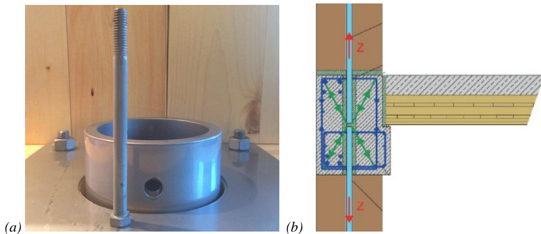
Figure 2-8: Novel connection detailing for structural robustness: (a) Brock Commons building (Photo credit Mpidi Bita); (b) HoHo building (Woschitz and Zotter, 2017) (Reprinted with permission)
