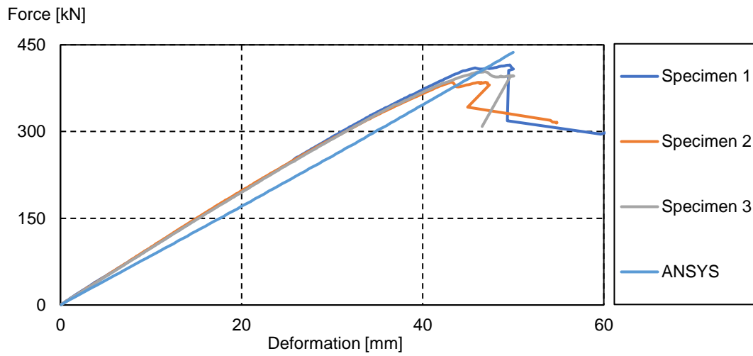
Figure A.1.2: (a) Deformed shape of the FE model of the point supported CLT floor; and (b) Comparison of load-deflection curves
