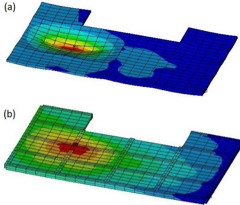
Figure 5-9: Top floor deformation after column B-3 removal: (a) M_1 model; and (b) M_2 Model
