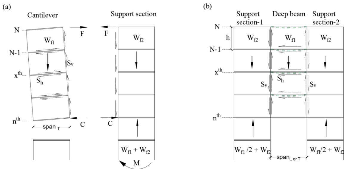
Figure 6-3: Wall system resistance mechanisms: (a) Cantilever action; (b) Beam action
