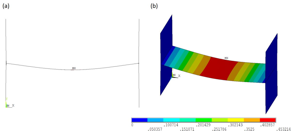
Figure 4-17: Deformed shapes of macro model: (a) Section view; and (b) Isometric view (in m)
