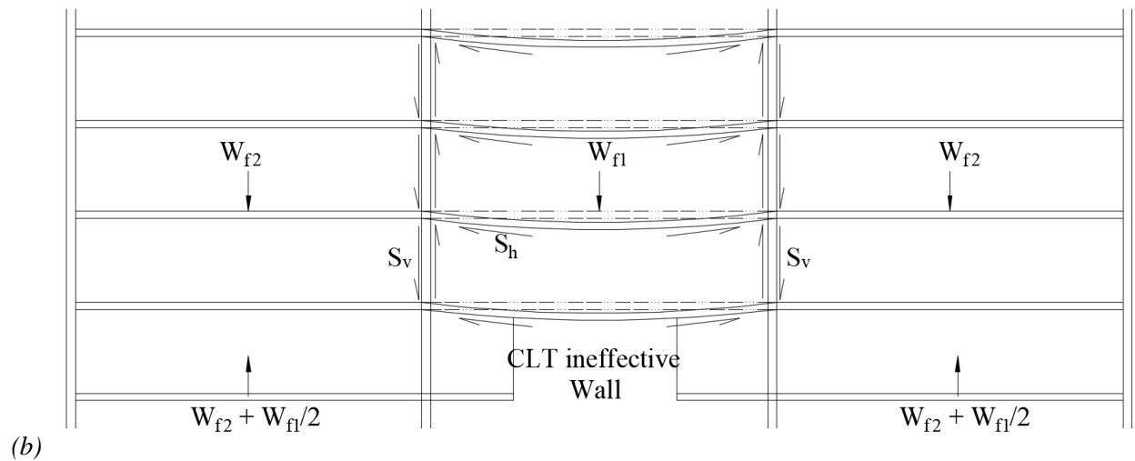
Figure 2-3: Wall system collapse-resistance mechanisms: (a) Cantilever action; and (b) Beam action (Schultz et al., 1977b)
