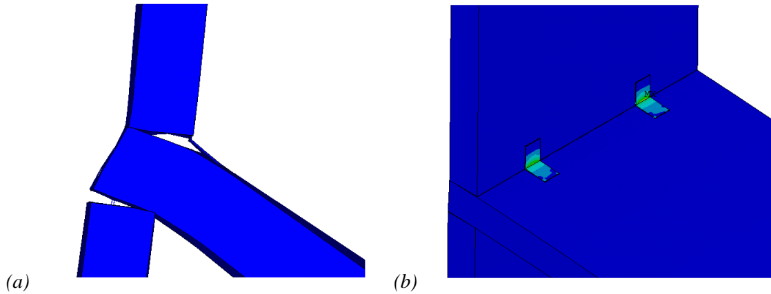
Figure 4-15: Failure of micro model: (a) Section view; and (b) Isometric view
