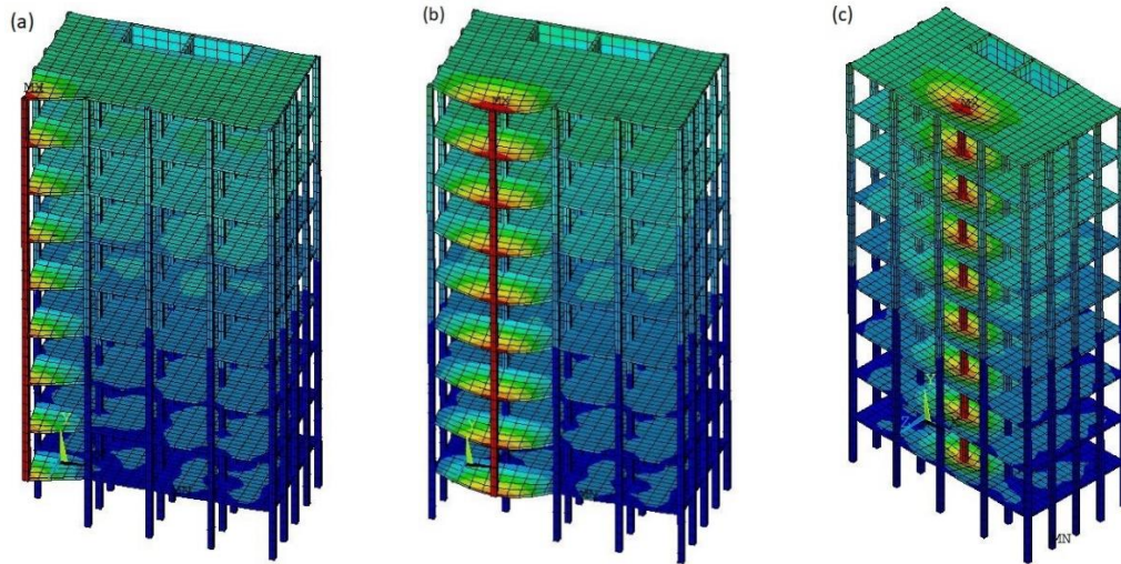
Figure 5-8: Deformed shape after column removal: (a) Column A-1; (b) Column B-1; and (c) Column C-
