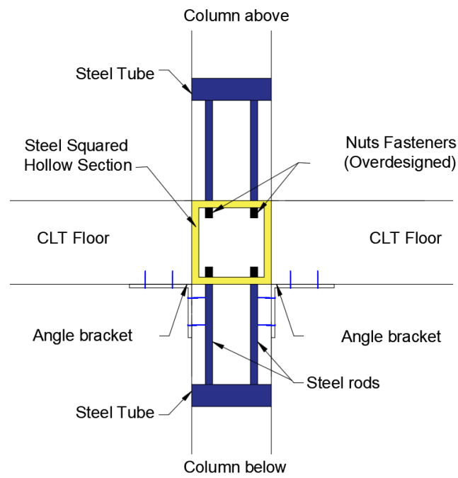
Figure 7-14: Detailing for hanging action for flat-plate mass-timber building: (a) Detailing-1 with HS and SS sections; (b) Detailing-2 with squared hollow section
