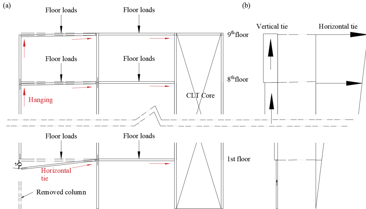
Figure 5-6: Alternative load-path: (a) Hanging action and tie-force; and (b) Idealised forces
