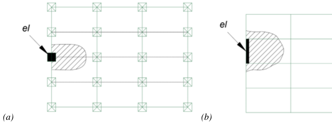
Figure 1-9: Acceptable collapse thresholds (CEN, 2006a): (a) Plan; and (b) Elevation
