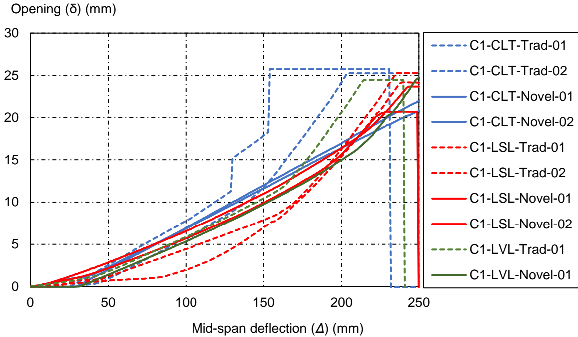
Figure 8-6: Axial deformation at the mid-span against applied deflection
