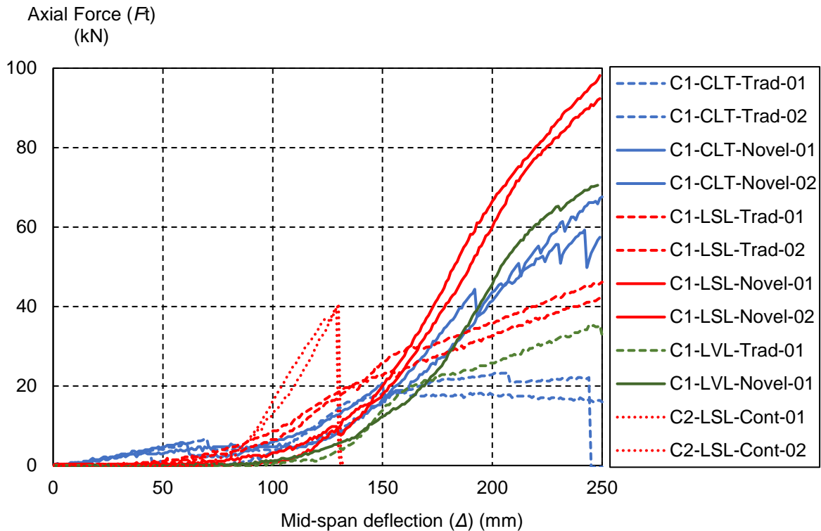
Figure 8-5: Axial tensile force against applied deflection
