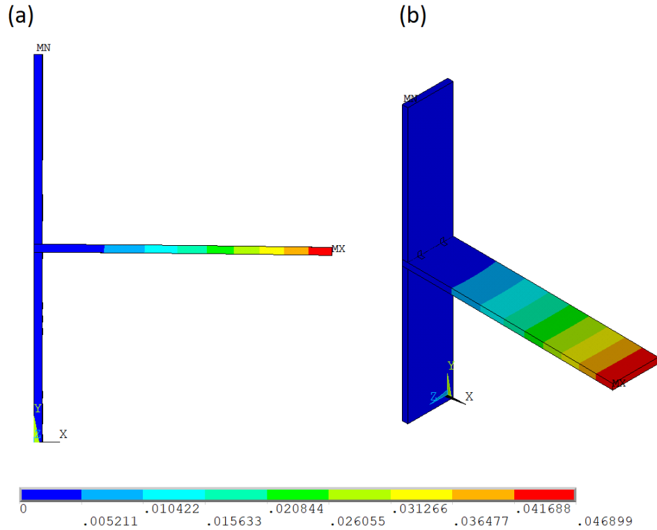
Figure 4-16: Deformed shape of the micro model: (a) Section view; and (b) Isometric view (in m)
