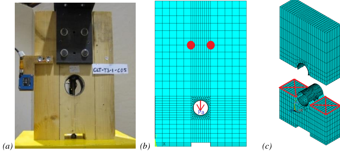
Figure 7-5: (a) Tube test specimen (Schneider, 2015) (Reprinted with permission); (b) FE model; and (c) CLT net tension failure
