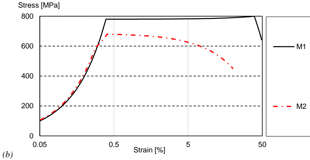
Figure 7-7: Material properties for steel tube ( M1 ) and welded area ( M2 ) (in logarithmic scale)
