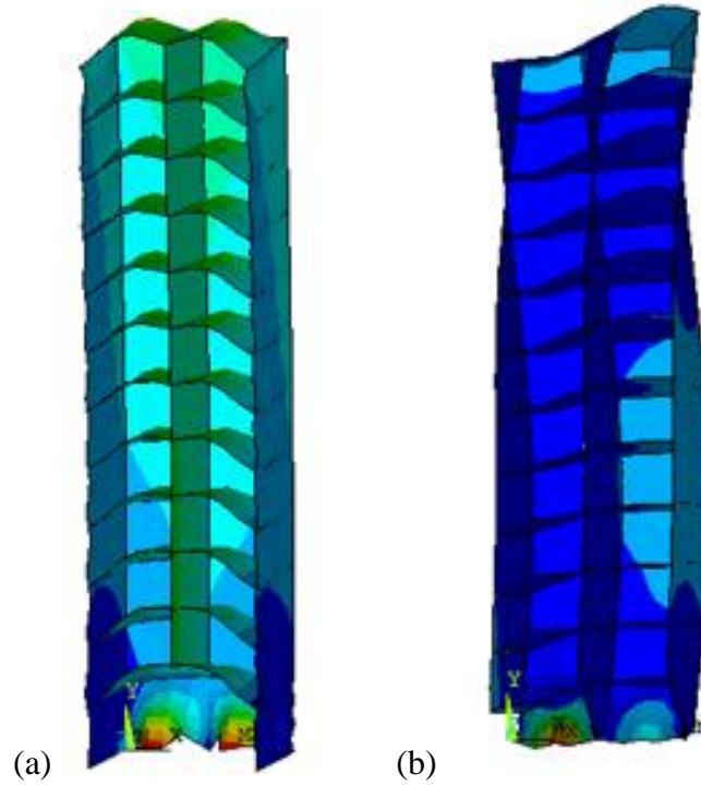
Figure 4-10: Mode shapes: (a) Internal removal; and (b) External removal
