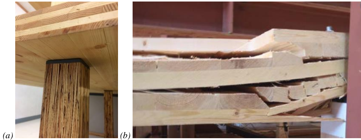
Figure 1-4: (a) Flat-plate mass-timber building (Photo credit Mpidi Bita); and (b) Rolling shear failure from experimental testing (Popovski et al., 2016) (Reprinted with permission)
