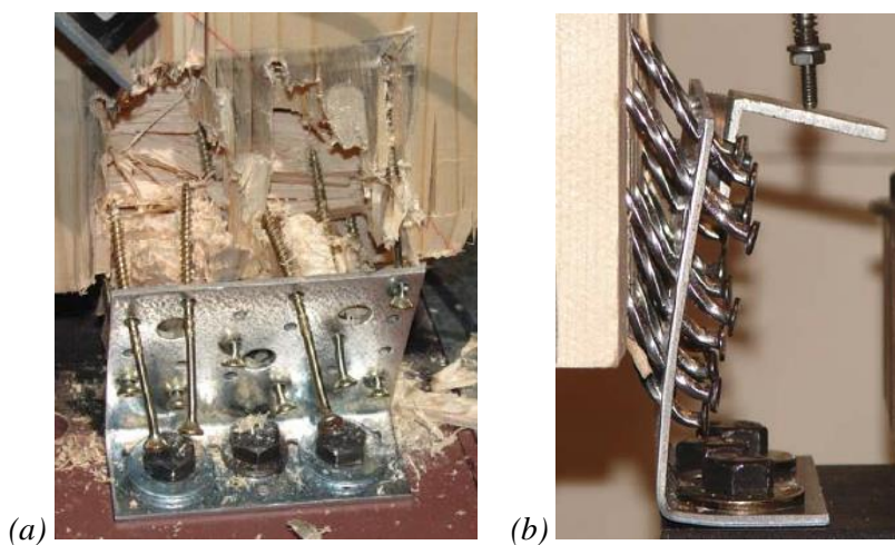
Figure 2-4: Damages of traditional non-robust and non-resilient connectors under reverse cyclic loads: (a) Brittle wood failure, and (b) Nails yielding (Schneider, 2015) (Reprinted with permission)
