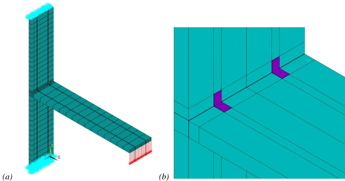
Figure 4-6: FE micro models: (a) Isometric view full; and (b) Zoomed isometric view
