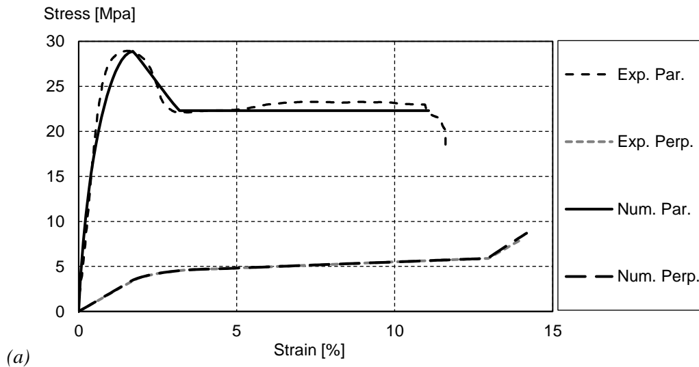
Figure 7-6: Experimental and numerical stress-strain curves for CLT
