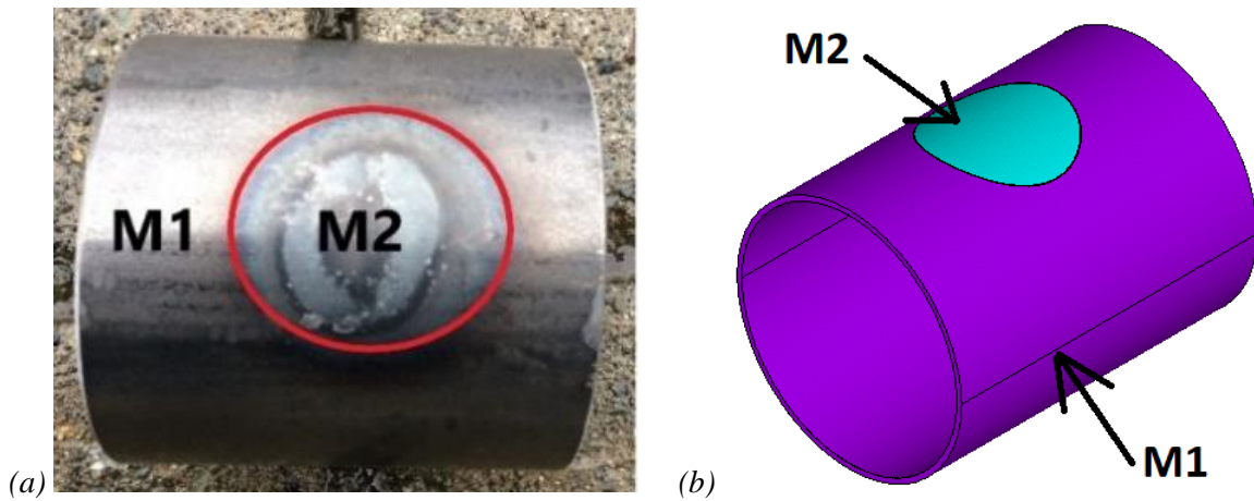
Figure 7-4: Steel tube zones with different material properties: (a) Tested tube (Photo credit Mpidi Bita); and (b) FE model
