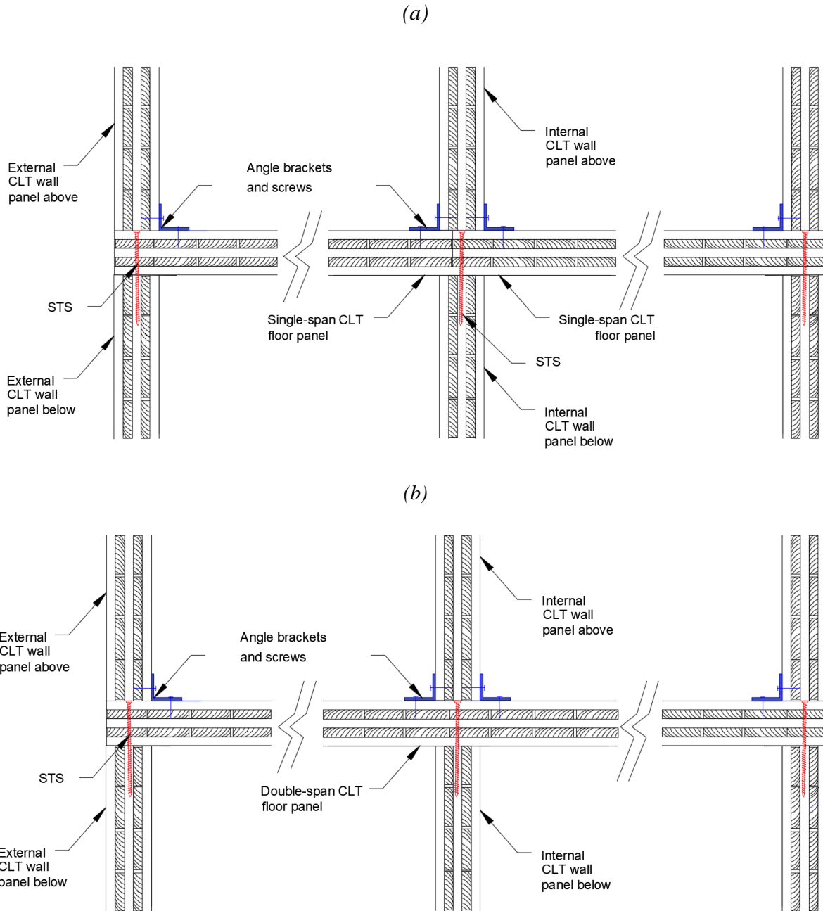
Figure 6-1: Connection detailing for platform-type CLT building: (a) Single span floor panel; and (b) Double span floor panel
