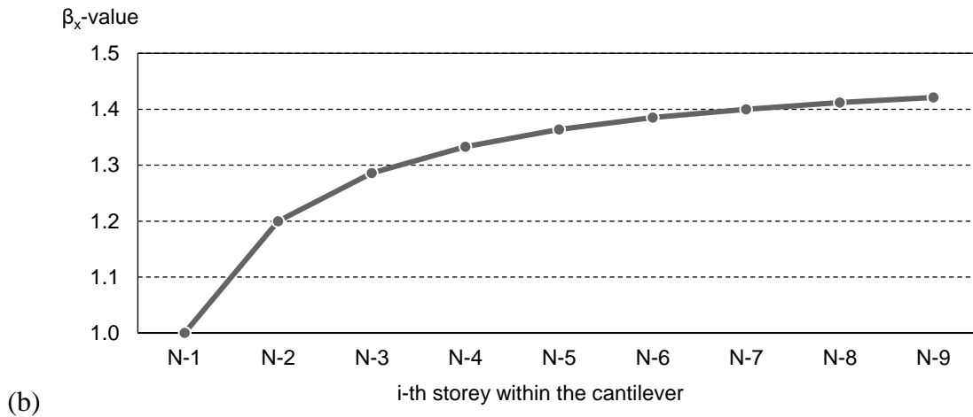
Figure 6-4: transverse tie forces at any storey for any cantilever size: (a) \alpha_x -values; and (b) \beta_x -values
