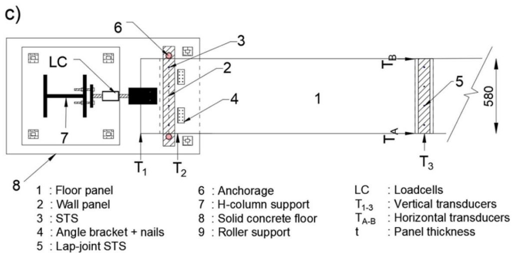
Figure 8-3: Test-setup: (a) Photo, (b) Elevation-view schematic, (c) Plan-view schematic
