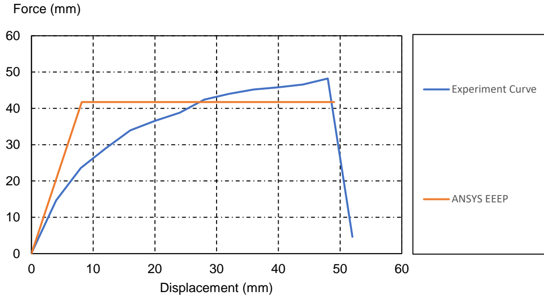
Figure A.4.1.2: Force against the applied deformation curves: Experimental results (Hossain et al., 2016) against EEEP curve used in Ansys model
