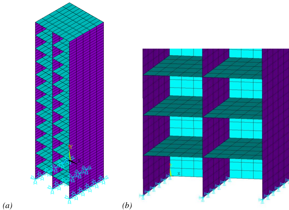
Figure 4-4: FE global model: (a) Isometric view full; and (b) Zoomed isometric view
