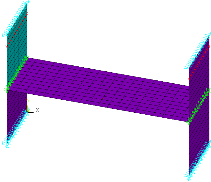
Figure 4-7: Isometric view of the macro model
