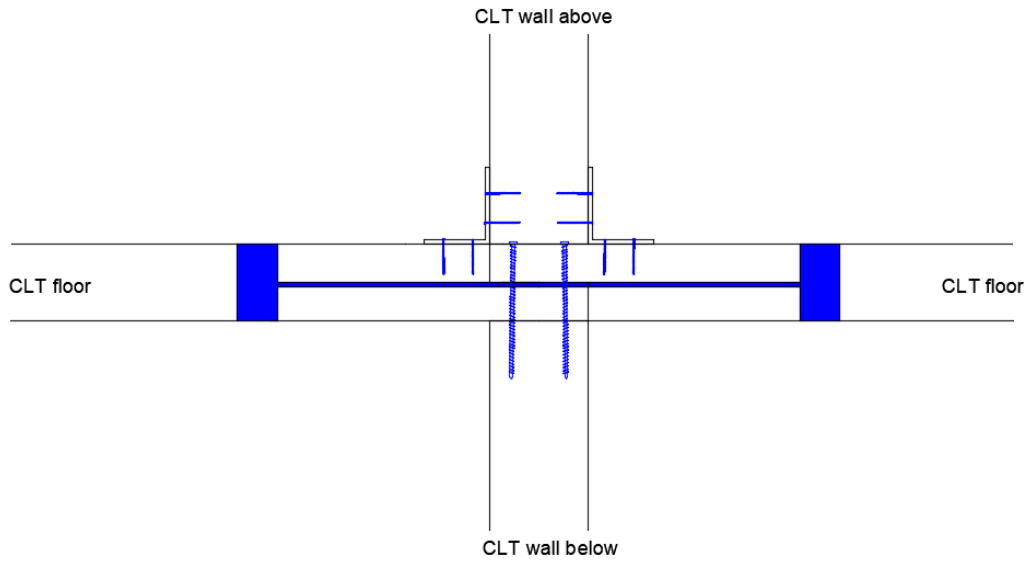
Figure 7-11: Detailing for catenary action for mass-timber platform-type and flat-plate constructions
