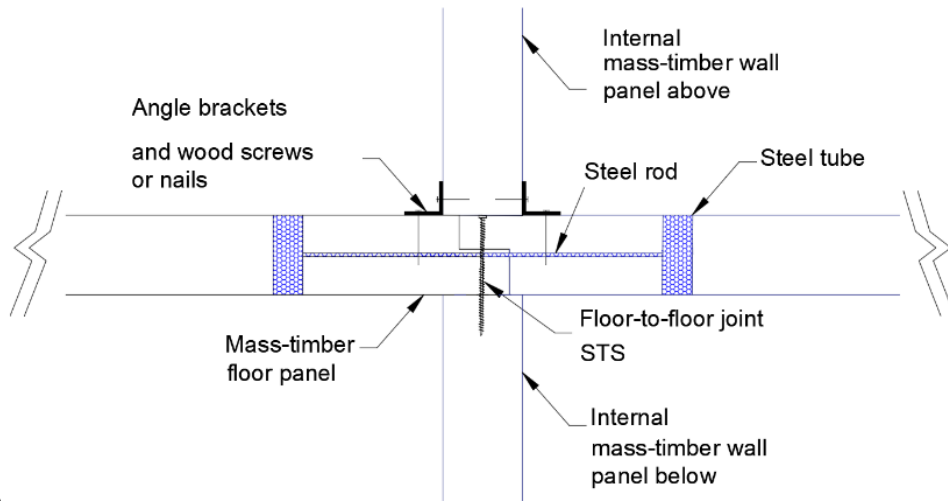
Figure 8-2: (a) Steel tube inserted in CLT panel; (b) Steel tubes and rods in mass-timber panel; and (c) Schematic representation of the detailing
