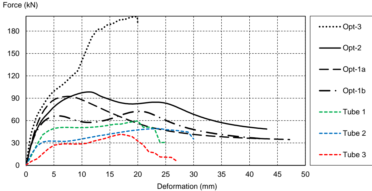
Figure 7-10: Numerical force vs deformation curves for optimised designs
