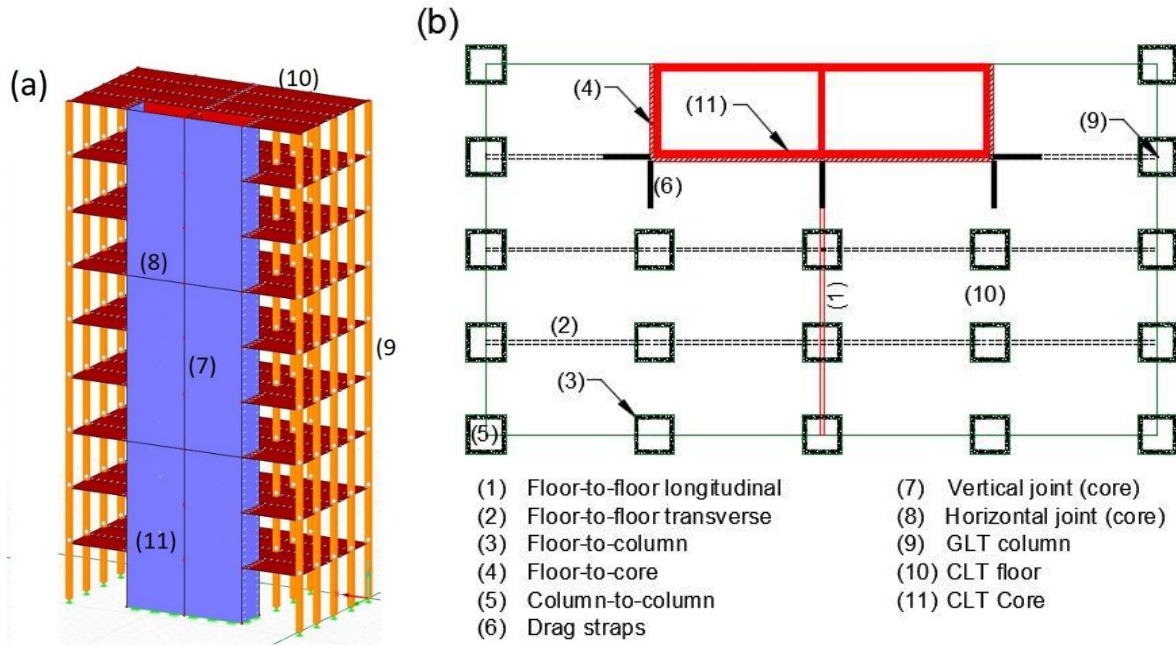
Figure 5-2: Main structural elements shown in: (a) Building isometric view; and (b) Floor plan
