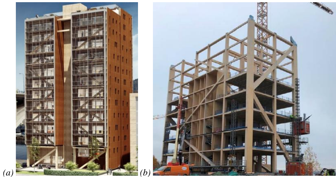
Figure 1-7: Post-and-beam construction: (a) Treet (Abrahamsen and Malo, 2014); and (b) Mjøstårnet (Abrahamsen, 2017) (Reprinted with permission)
