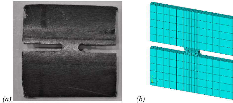
Figure 7-3: Bone-shaped steel specimens: (a) Experiment specimen (Photo credit Mpidi Bita); and (b) FE model specimen
