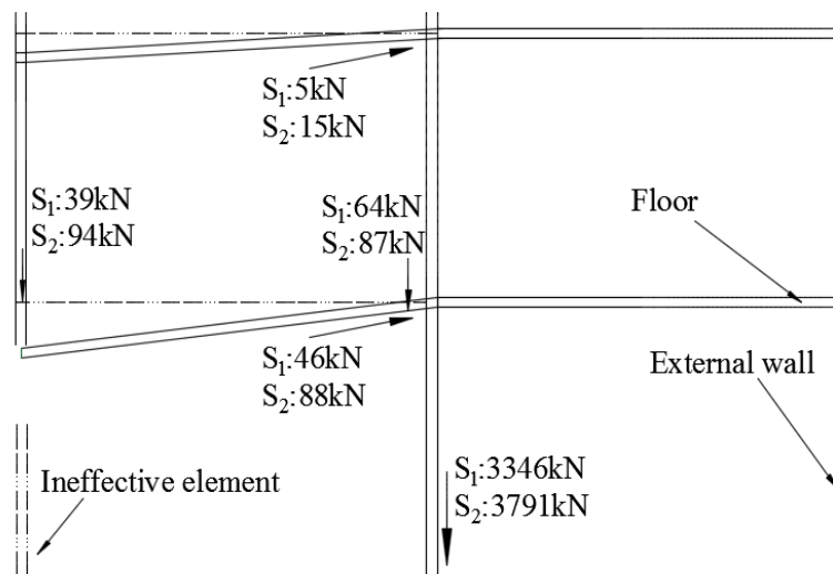
Figure 4-14: Results of external wall removal
