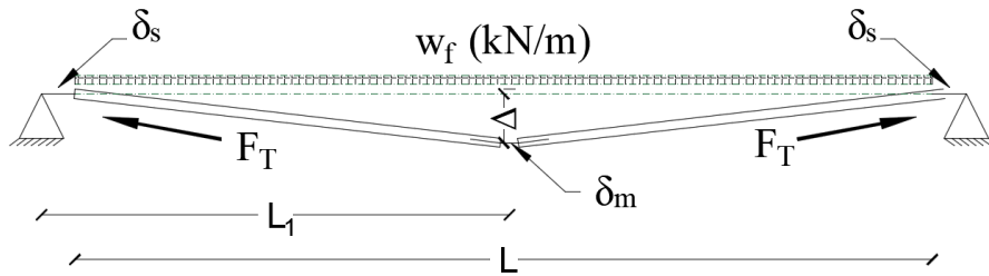
Figure A.2.1.1: 2D Schematic representation of floor catenary action
