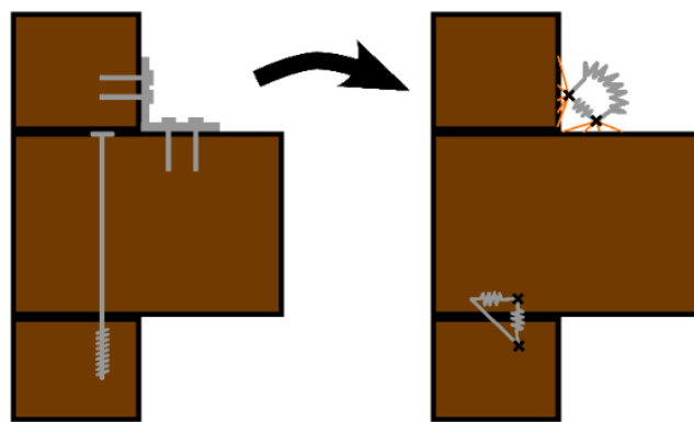
Figure 2-6: Modelling assumptions: Replacement of connection components with connector elements (Huber et al., 2018a) (Reprinted with permission)
