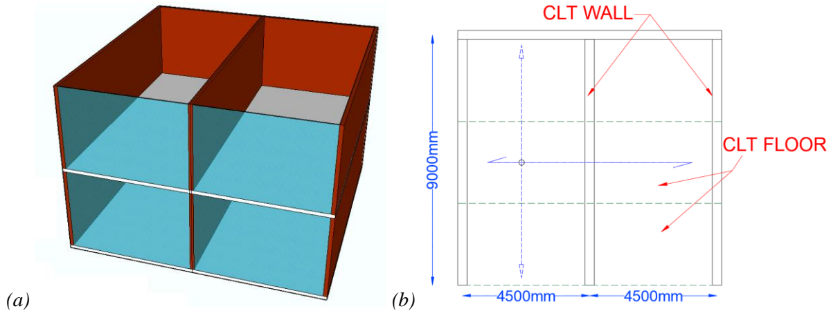
Figure 4-1: TRADA building: (a) Schematic isometric view; (b) Floor plan view
