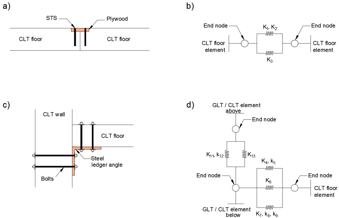
Figure 5-3: Floor-to-floor spline connection: (a) Sketch, (b) Springs idealisation; and Floor-to-steel ledger angle: (c) Sketch, (d) Springs idealisation
