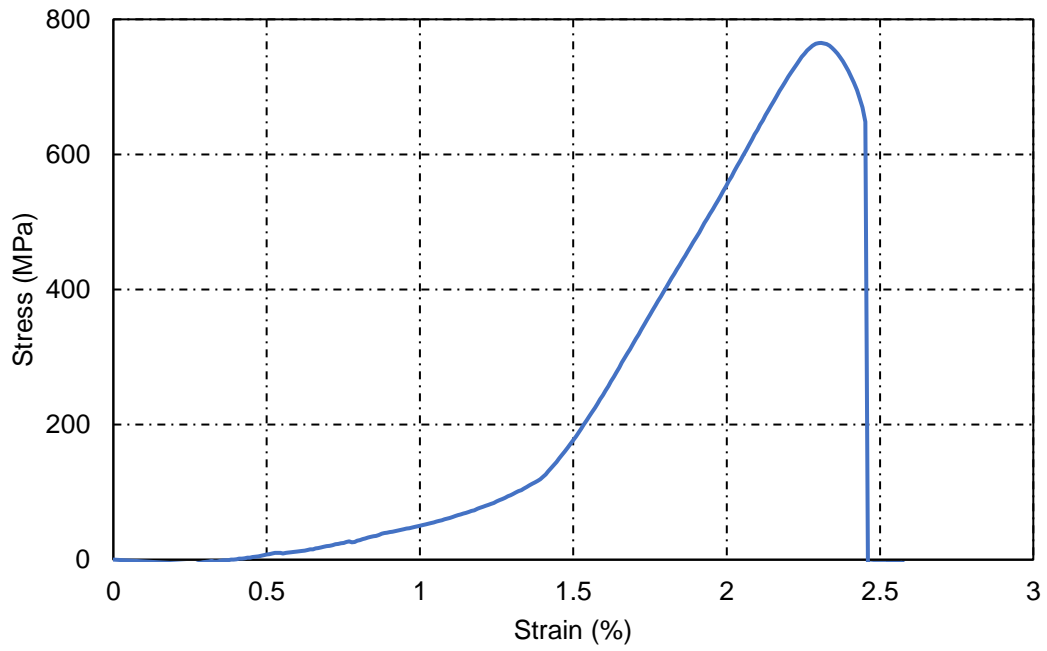
Figure A.5: Experimental results of bone-shape steel specimens: Stress vs Strain curve
