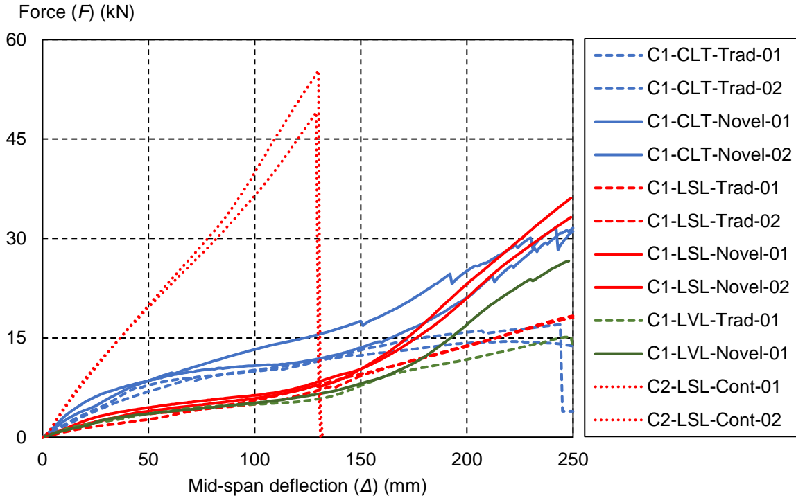
Figure 8-4: Force against applied deflection
