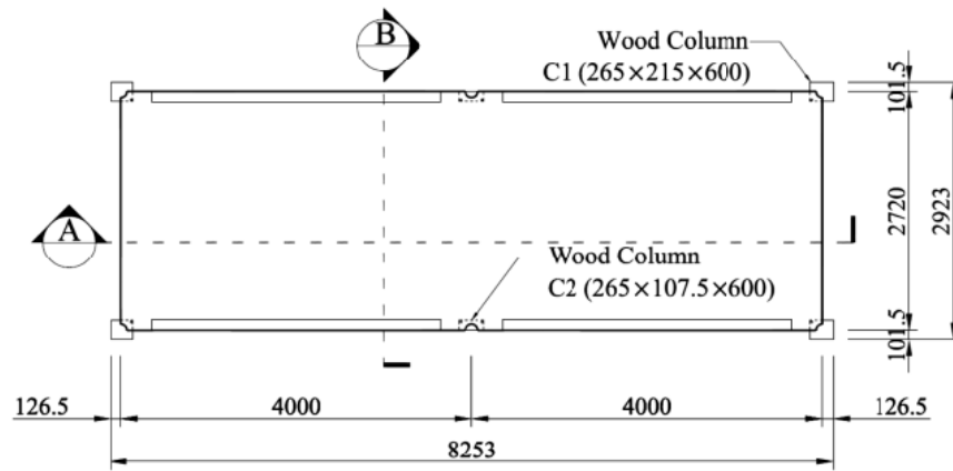
Figure A.1.1: Plan view of the tested point supported CLT floors (Popovski et al., 2016)
