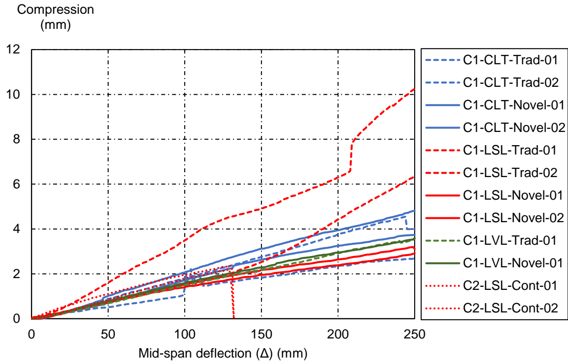
Figure 8-7: Compression at the point of rotation of the floor against applied deflection
