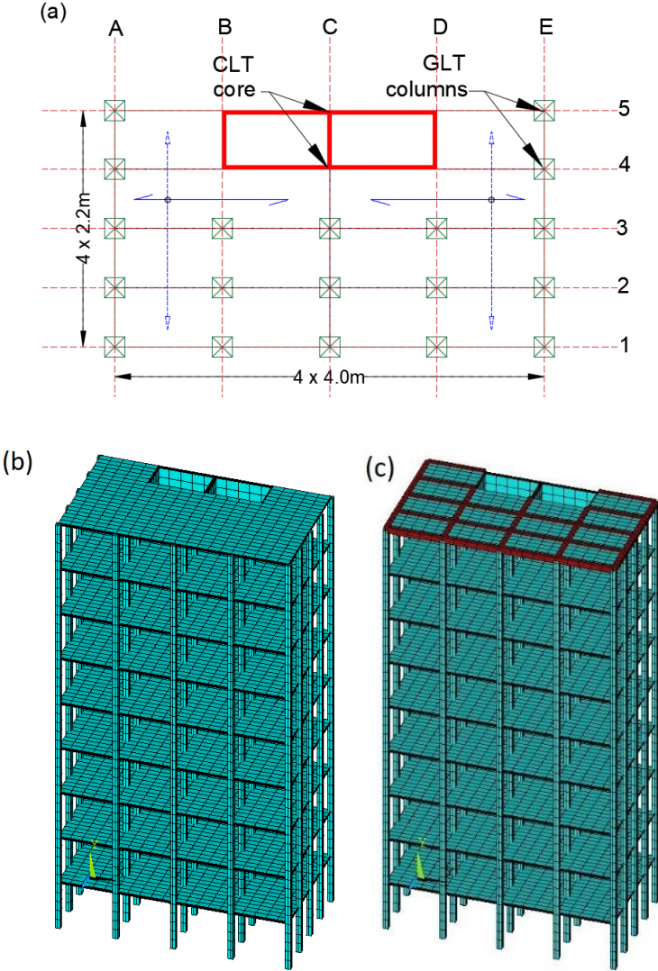
Figure 5-1: Case study building: (a) Building floor plan; (b) Isometric view of numerical original ( M_1 ) model; and (c) Isometric view of numerical improved ( M_2 ) model
